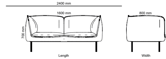
Divided 2-seated & 3-seated sofa
